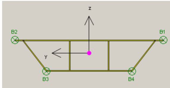
Steel box section for the deck
