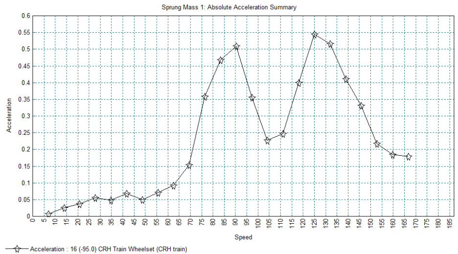
(Sixteenth spring-mass system)
