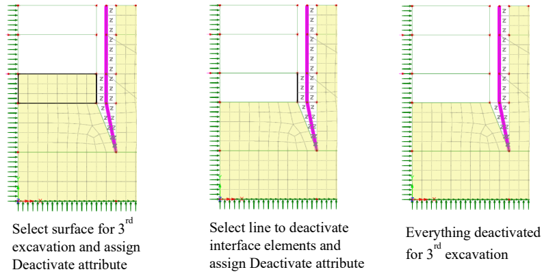
Figure 56: 3 rd Excavation
