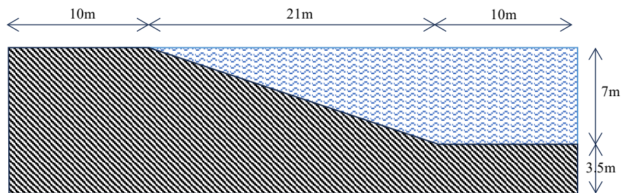
Model geometry
