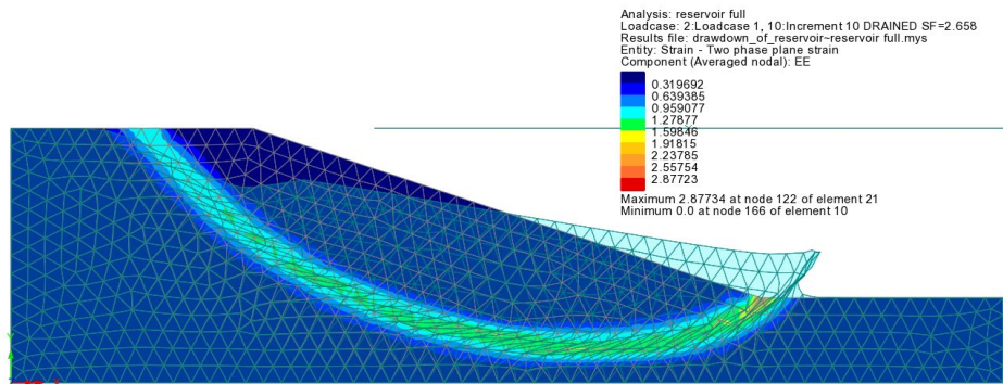
Full reservoir – drained – SF =2.66
