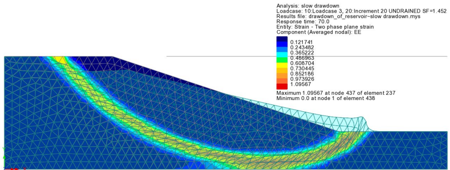
Slow drawdown – undrained – SF = 1.45
