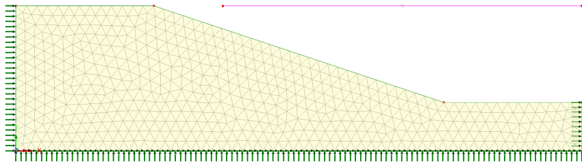
Boundary conditions
