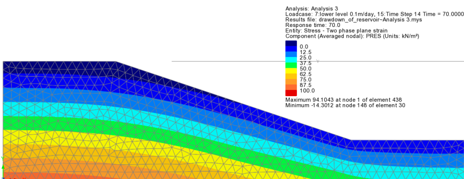
Day 70: Slow drawdown 0.1m/day
