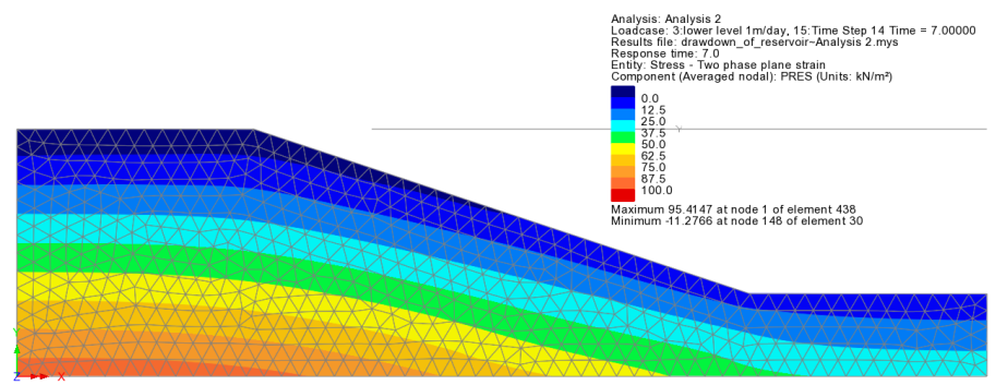
Day 7: Fast drawdown 1m/day
