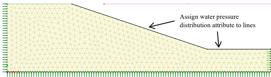
Assignment of water pressure distribution attribute
