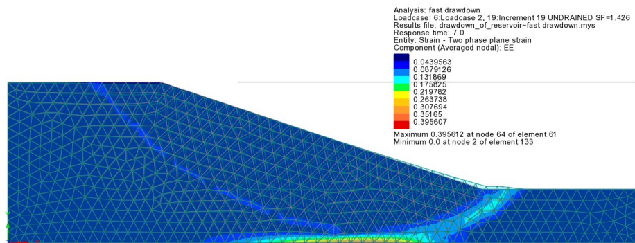
Fast drawdown – undrained – SF = 1.43
