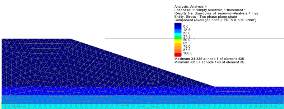
Empty reservoir
