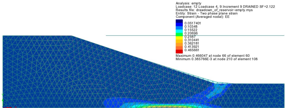
Empty reservoir – drained – SF = 2.12
