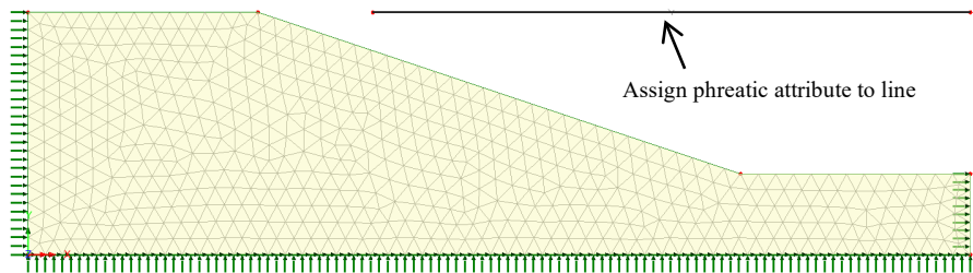
Assignment of phreatic attribute
