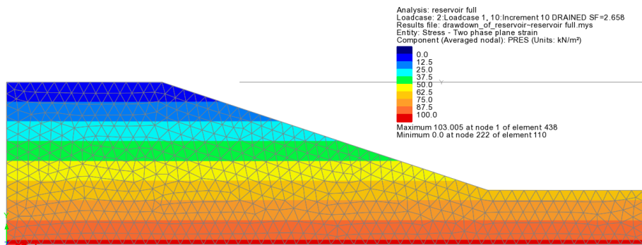
Full reservoir
