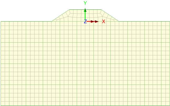
Figure 3: Model meshing
