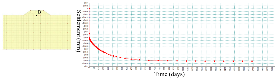
Figure 12: Settlement at point B
