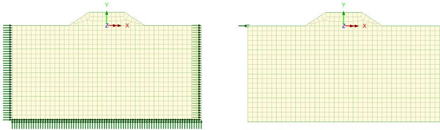
Figure 5: Boundary conditions
