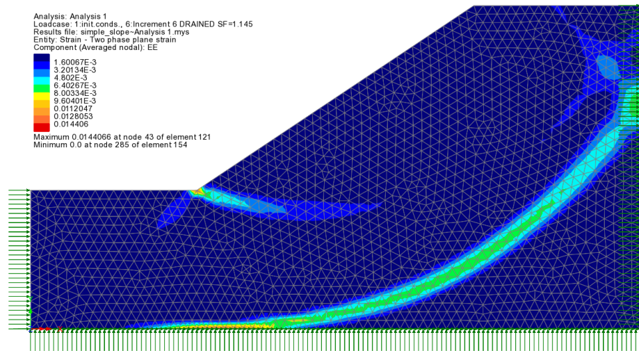
Effective strain at safety factor 1.145
