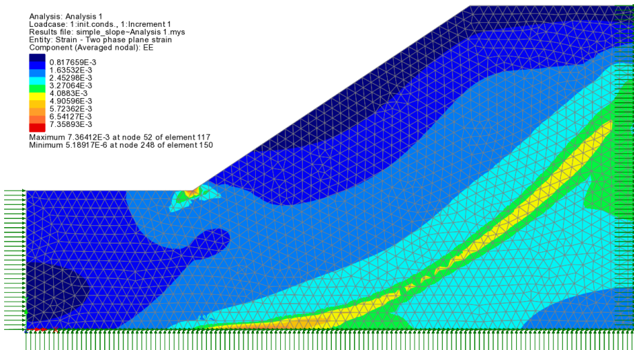
Effective strain at safety factor 1.0
