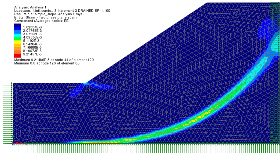
Effective strain at safety factor 1.1
